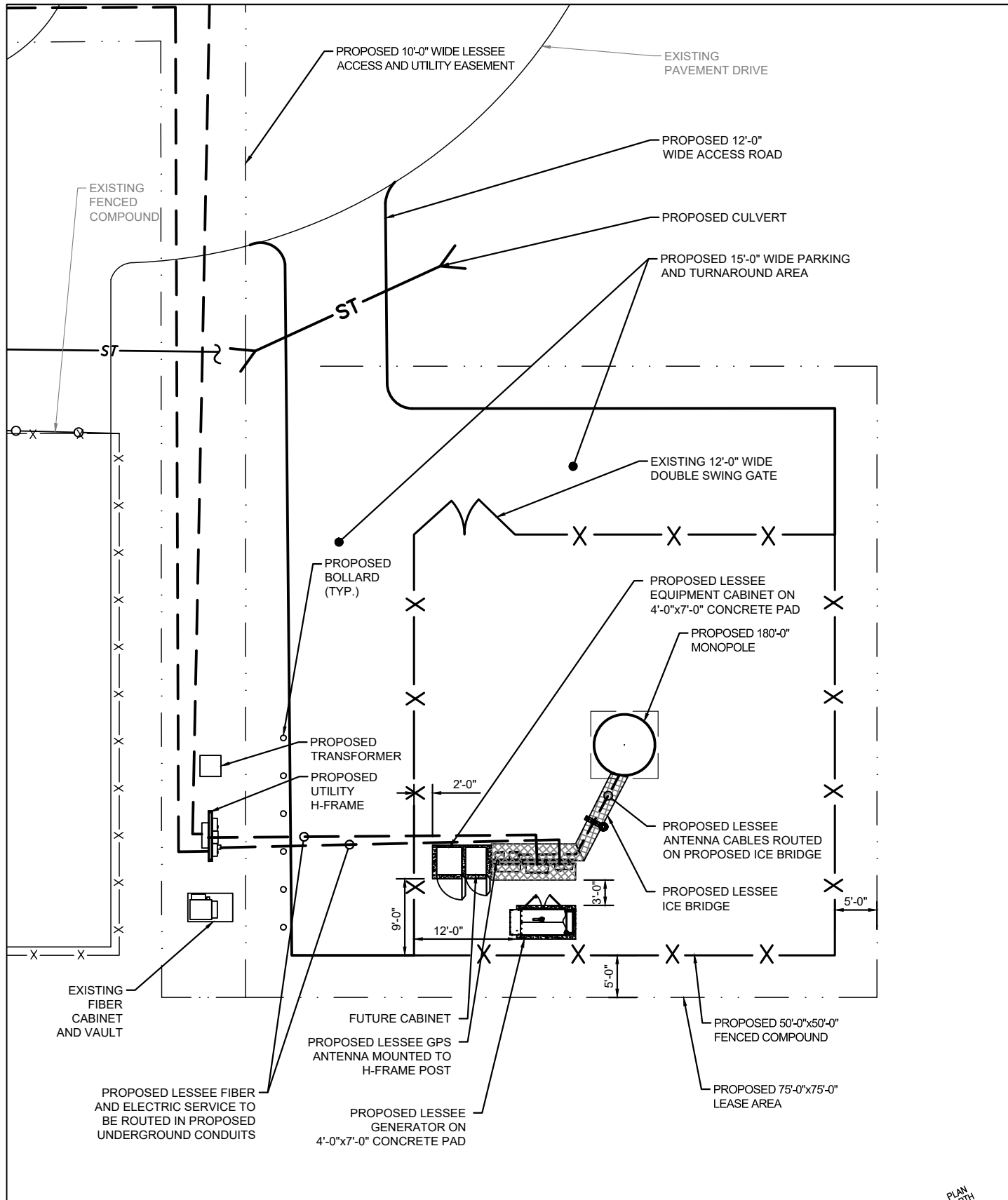
EQUIPMENT LAYOUT PLAN SCALE: 1" = 16'-0"
