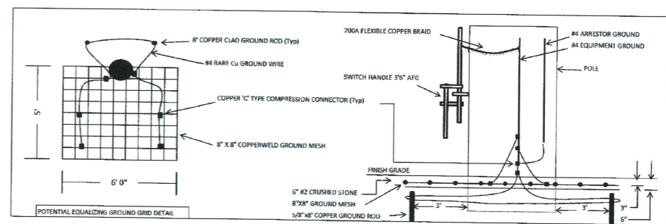
SECTION OF POLE LINE & GROUNDING DETAILS FOR GOAB/METERING POLE NO SCALE
